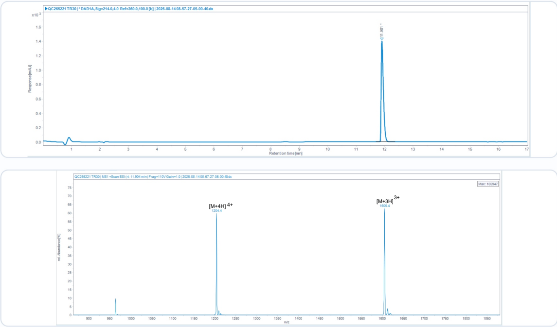
HPLC Chromatogram · Retention Time 11.901 min
